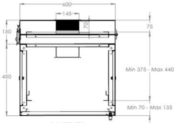
MAX/MIN EQUIPMENT MOUNTING DISTANCE
