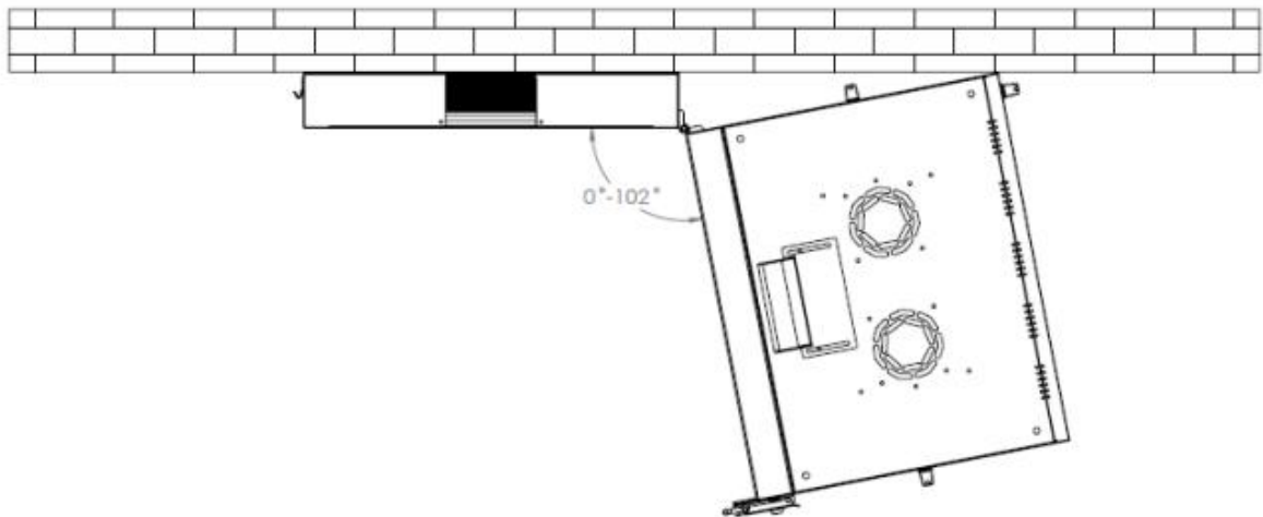
DOUBLE SECTION OPENING ANGLE
