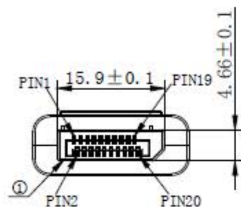
DisplayPort Male
