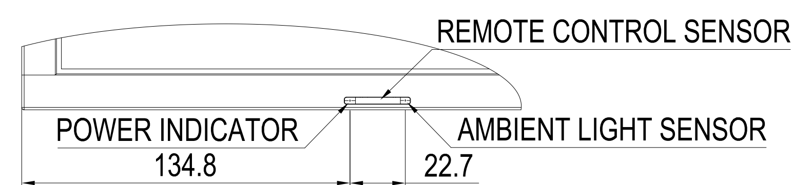
DETAIL C SCALE 3:1
