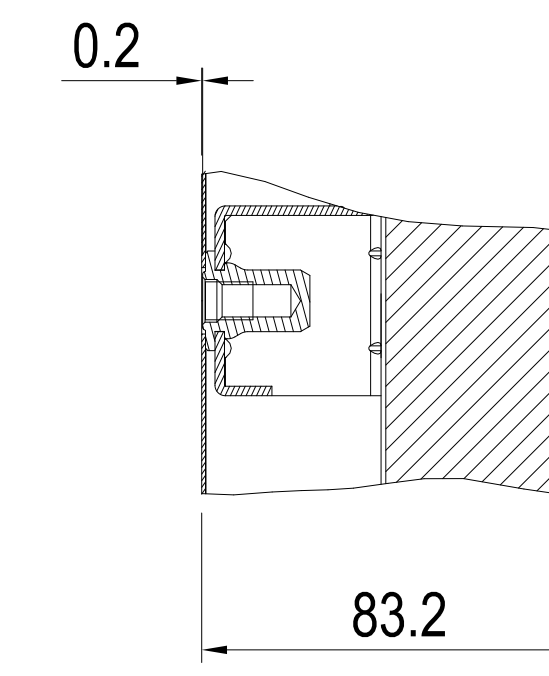
SECTION B-B SCALE 3:1
