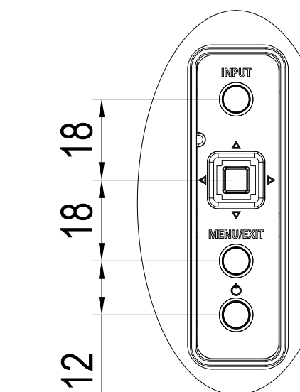
DETAIL E SCALE 4:1
