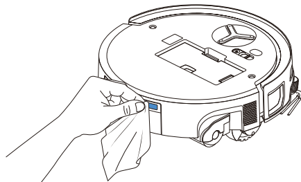
Clean Charging Contacts
